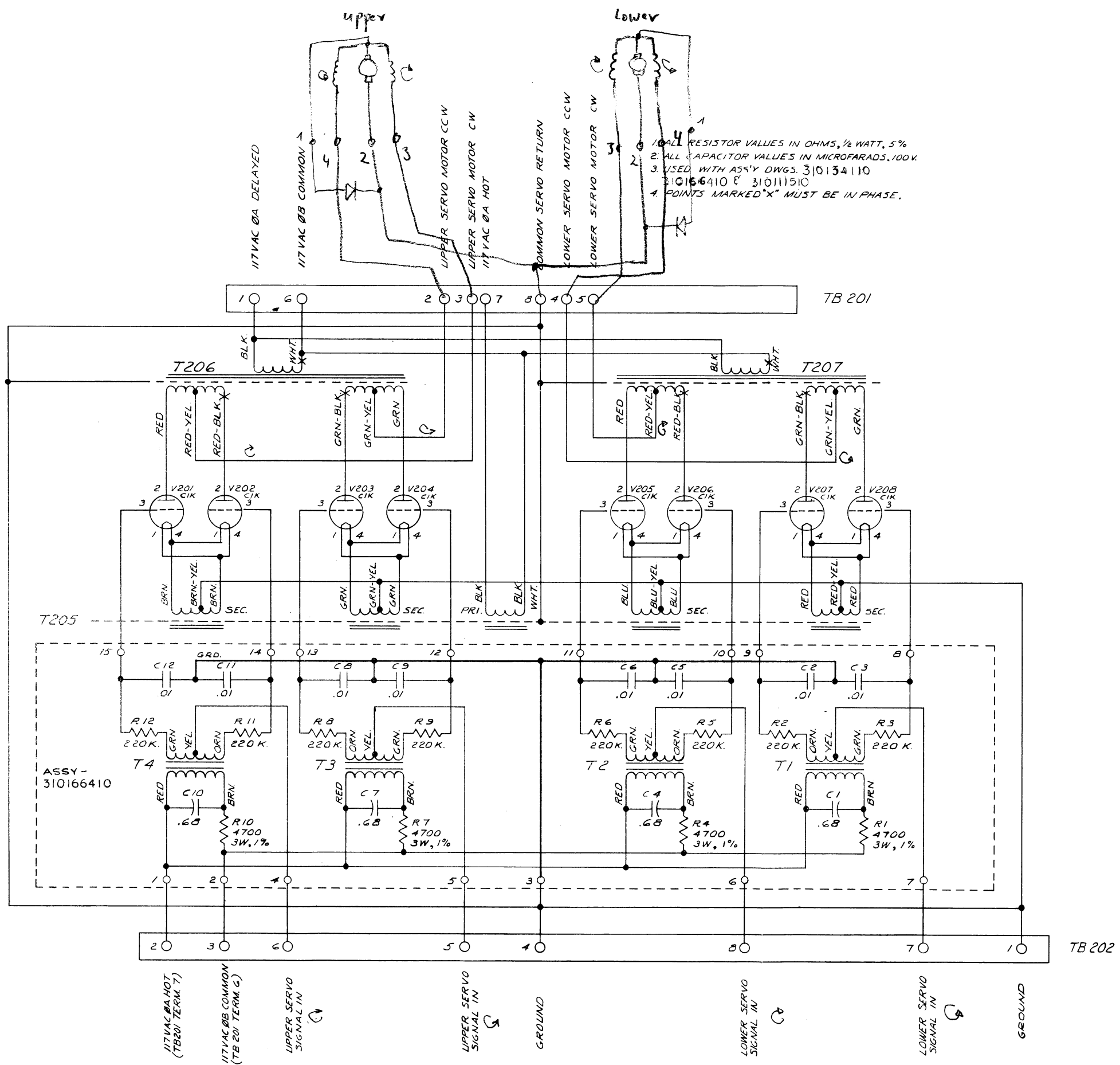
Figure 8-9 Schematic Diagram, Servo Motor Power Supply PS-200
