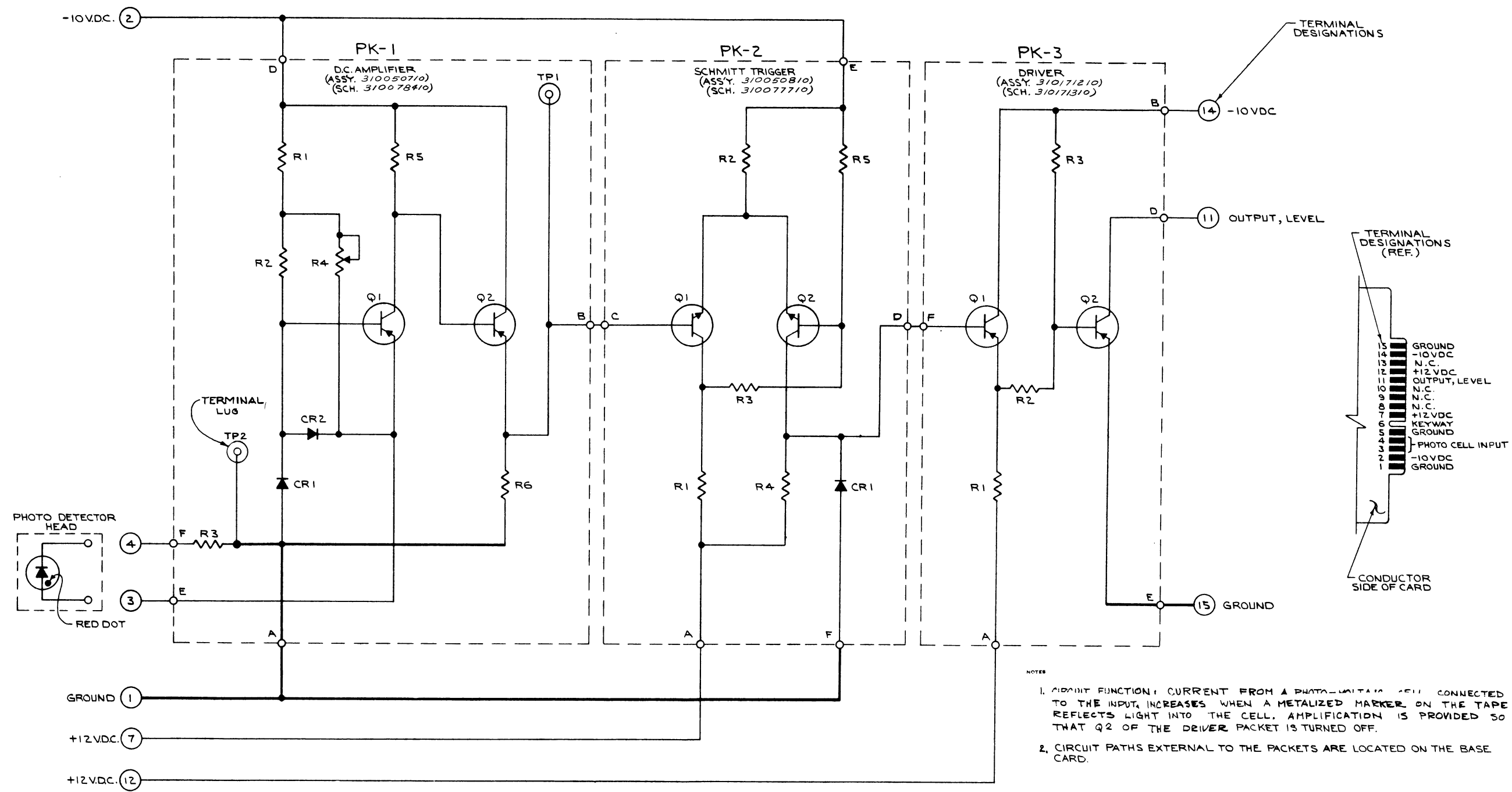
Figure 8-14 Schematic Diagram, Photosense Base Card (Used with Photosense Kit 31 01082 10)
