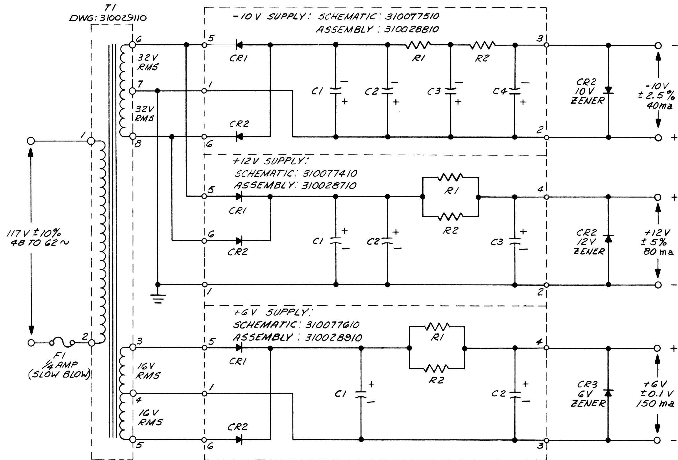
Figure 8-15 Schematic Diagram, Photosense Power Supply
