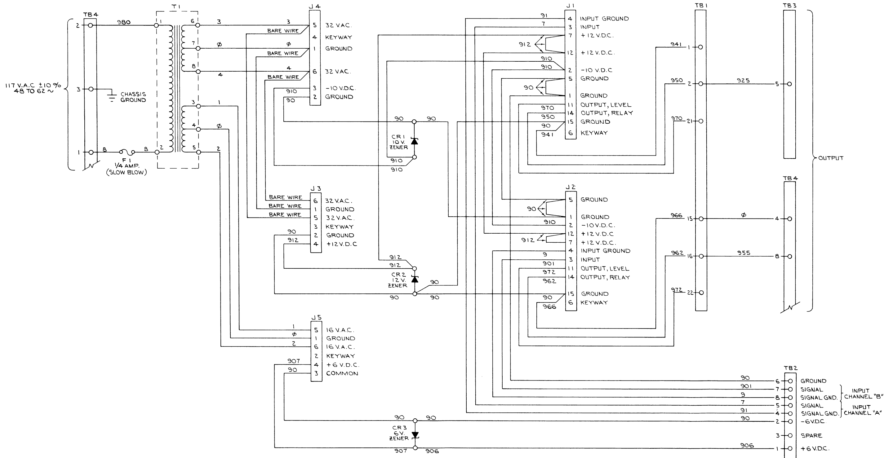
Figure 8-17 Schematic Diagram, Photosense Chassis Wiring (Used with Photosense Kit 31 01082 10)
